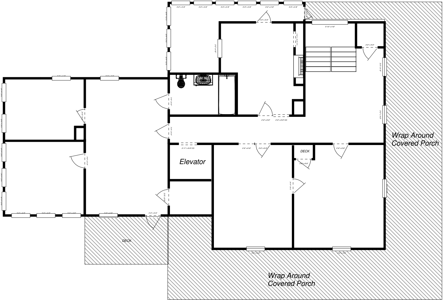
2nd Floor
